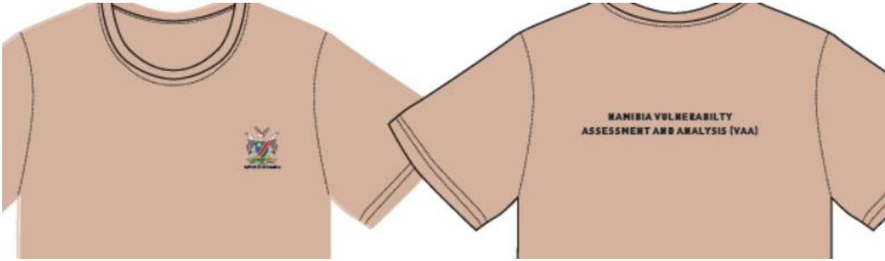
Figure 3: Tshirts design
