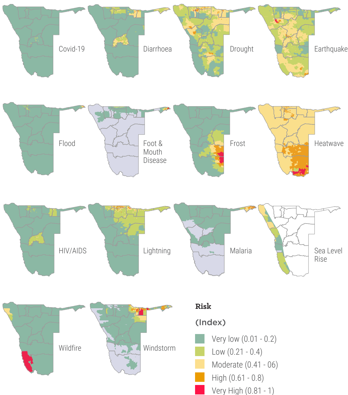
Figure 111: Spatial distribution of the risks to natural hazards covered in this study
