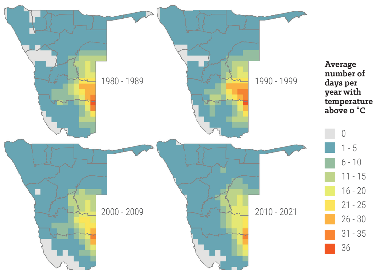
Figure 51: Average number of days per year with temperature below 0 °C from 1980 to 2021 (data source: NOAA)
