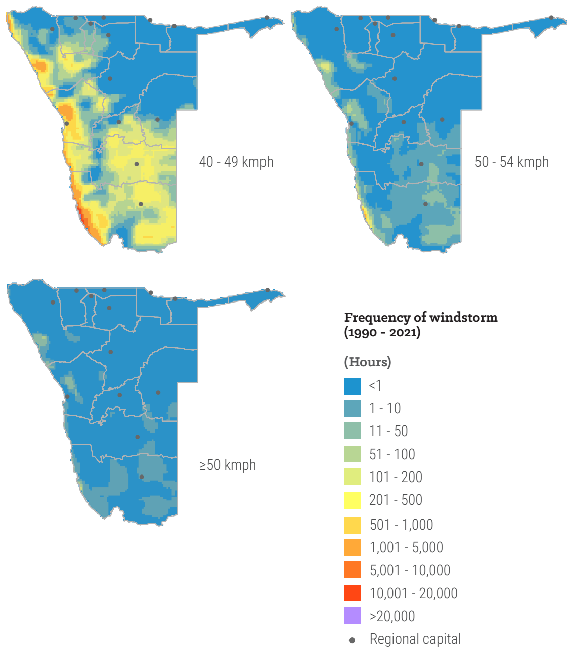
Figure 55: Frequency of sandstorms of various speeds from 1990 to 2021 based on the ERA5-Land hourly dataset
